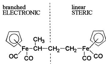
Scheme 4. Linear versus branched reactivity.
