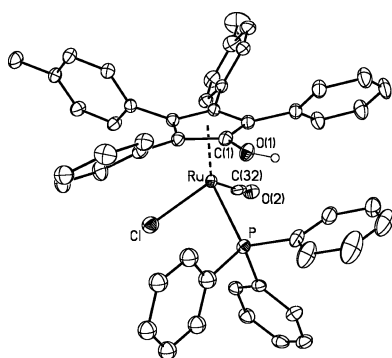
Figure 3. X-ray crystal structure of 7 . Selected bond lengths (Å) and angles (deg): Ru–P, 2.3423(13); P–Ru–Cl, 86.73(5); C(32)–Ru–Cl, 93.09(16); C(32)–Ru–P, 89.79(14); P–Ru–C(1)–O(1), 1.2(4); Cl–Ru–C(1)–O(1), 89.0(4).
