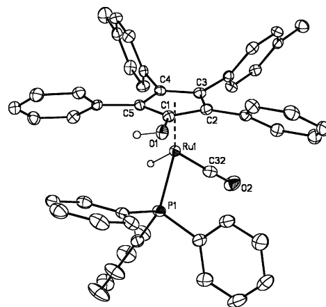
Figure 4. X-ray crystal structure of 8 . Selected bond lengths (Å) and angles (deg): Ru(1)–P(1), 2.2792(10); P(1)–Ru(1)–H(1), 81.6(13); C(32)–Ru(1)–H(1), 78.6(13); C(32)–Ru(1)–P(1), 88.18(13); P(1)–Ru(1)–C(1)–O(1), 8.9(3); C(32)–Ru(1)–C(1)–O(1), 90.0(4).
