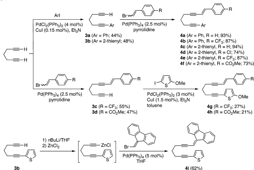
SCHEME 1. Synthesis of 4a–i
