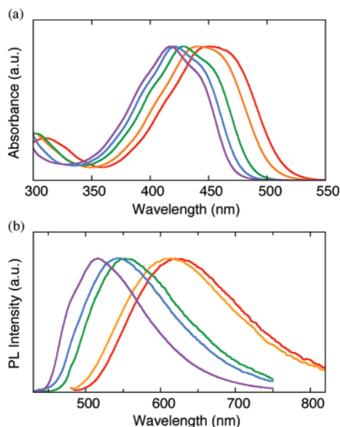
FIGURE 2. UV-vis absorption spectra (a) and fluorescence spectra (b) of 5c , 5e–h in THF. The peak maxima are normalized. The color: 5c , purple; 5e , blue; 5f , green; 5g , orange; 5h , red.
