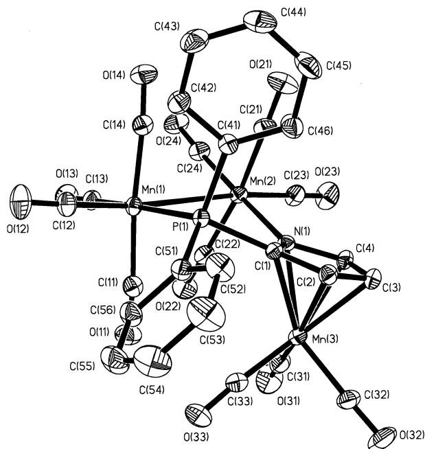
Fig. 1. Molecular structure of the cluster [\text{Mn}_3(\mu_3\text{-P}, N, \eta^5\text{-Ph}_2\text{PC}_4\text{H}_3\text{N})(\text{CO})_{11}] .
