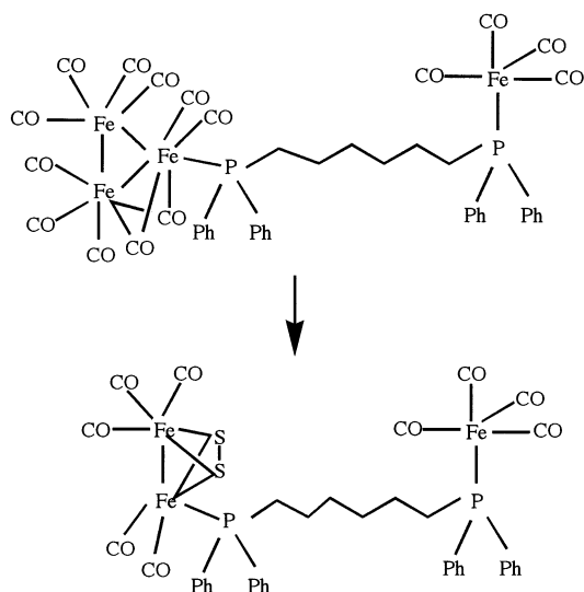
Scheme 1. Proposed reaction scheme for the formation of compounds with formulae [\{\text{Fe}_2\text{S}_2(\text{CO})_5\}_2\text{Ph}_2\text{P}(\text{CH}_2)_n\text{PPh}_2[\text{Fe}(\text{CO})_4]] .
