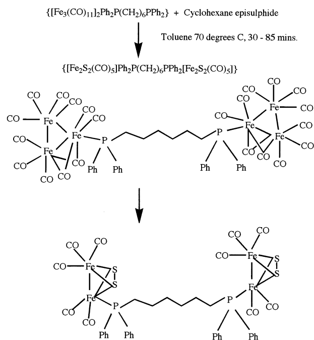
Scheme 2. Proposed reaction scheme for the formation of compounds with formulae \{[\text{Fe}_2\text{S}_2(\text{CO})_5]_2\text{Ph}_2\text{P}(\text{CH}_2)_n\text{PPh}_2\} .
