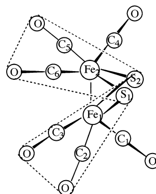
Fig. 3. Geometrical representation of [\text{Fe}_2\text{S}_2(\text{CO})_6] .
