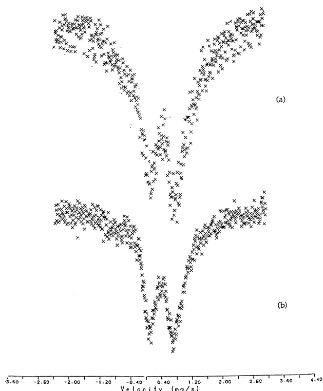
Fig. 2. Mössbauer spectra of compounds with formula \{[\text{Fe}_2\text{S}_2(\text{CO})_5]_2\text{Ph}_2\text{P}(\text{CH}_2)_n\text{PPh}_2\} (a) n = 6 ( 10 ) and n = 3 ( 4 ).
