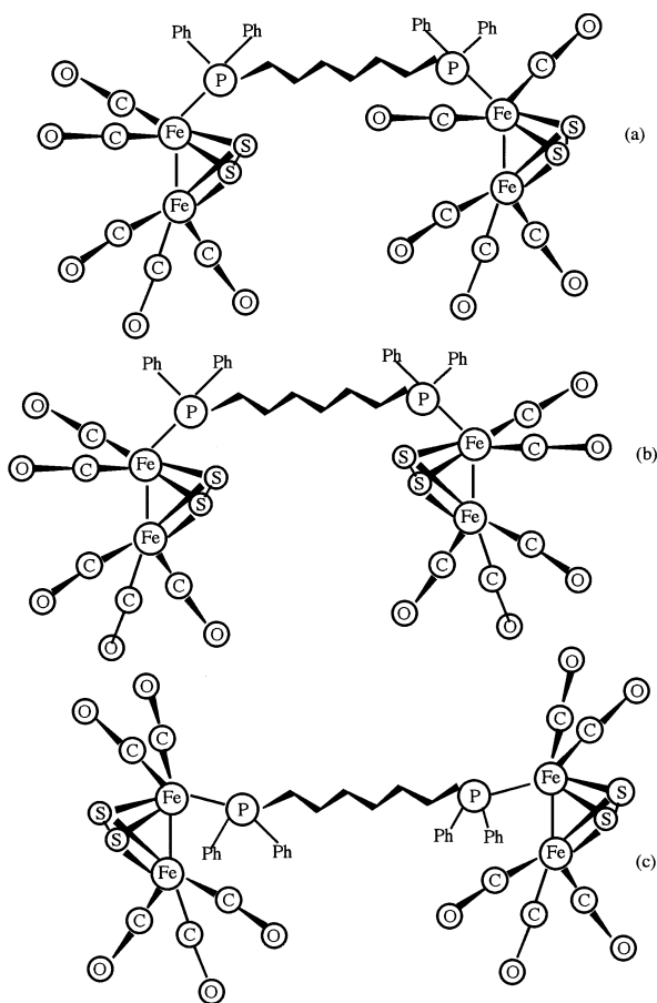
Fig. 4. Possible combinations of two [\text{Fe}_2\text{S}_2(\text{CO})_6] units; (a) apical to basal, (b) apical to apical and (c) basal to basal.
