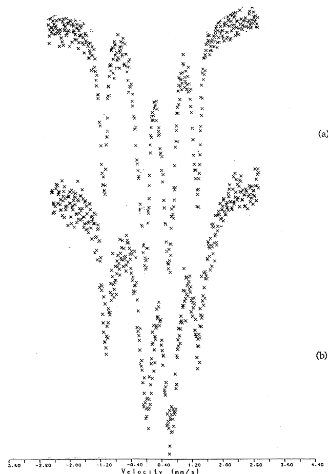
Fig. 1. Mössbauer spectra of compounds with formula [\{\text{Fe}_2\text{S}_2(\text{CO})_5\}_2\text{Ph}_2\text{P}(\text{CH}_2)_n\text{PPh}_2[\text{Fe}(\text{CO})_4]] (a) n = 4 ( 2 ) and (b) n = 6 ( 3 ).
