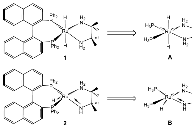
Figure 2. Simplification made for 1 and 2 for the calculation of the structures shown in Scheme 1.
