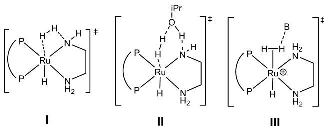
Figure 1. Three transition states proposed by Noyori and co-workers (ref 25) for the formation of the trans -dihydride in the presence of added KOtBu (I or II) and in the absence of added KOtBu (III) where the base is proposed to be the alcohol solvent. P–P is ( S )-tolbinap and the diamine is ( S,S )-dppe.
