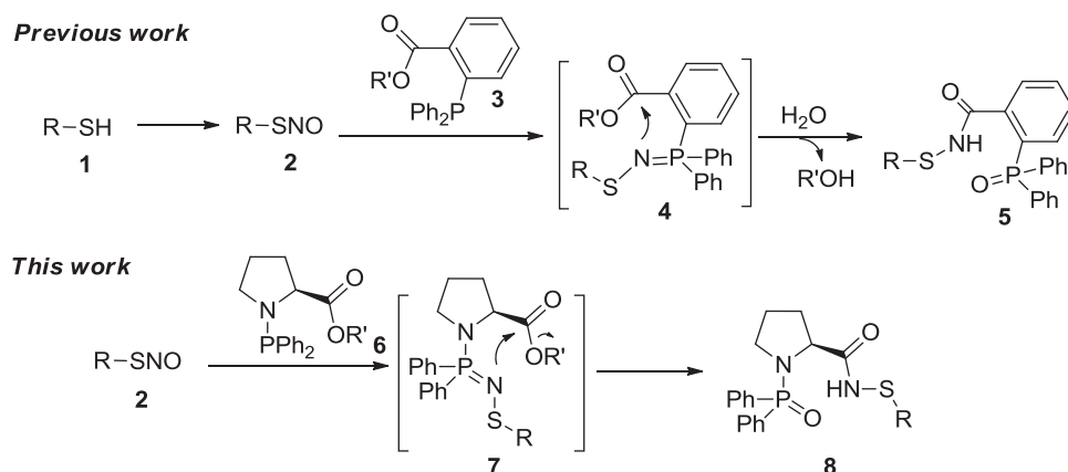
Scheme 1 Reductive ligations of S -nitrosothiols.
