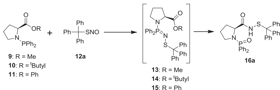
Scheme 2 Reactions between proline-based phosphoramidites and TrSNO.
