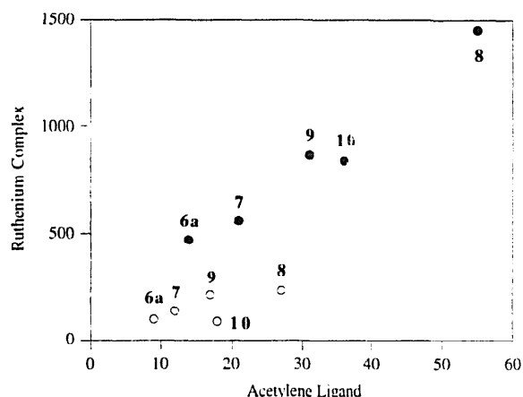
Fig. 3. Correlation of molecular quadratic hyperpolarizabilities of complexes 6a , 7–10 with those of the corresponding terminal alkynes ( 10^{-30} \text{ cm}^5 \text{ esu}^{-1} ); (●) experimental; (○) two-level corrected.
