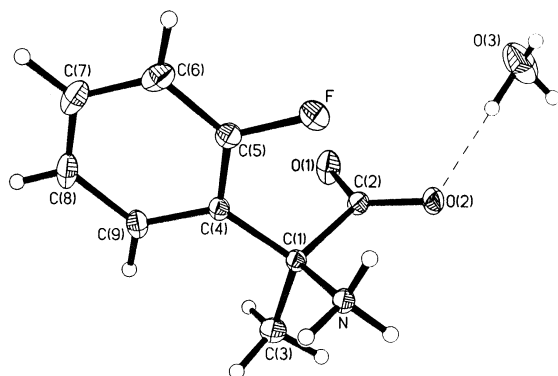
Fig. 2. Molecular structure of 8c·H 2 O . Selected bond lengths (Å) and angles (°): C(1)–C(2) 1.563(2), C(1)–C(3) 1.521(2), C(1)–C(4) 1.522(2), C(1)–N 1.502(2), C(2)–O(1) 1.235(2), C(2)–O(2) 1.249(2); N–C(1)–C(2) 108.1(1), N–C(1)–C(3) 107.1(1), N–C(1)–C(4) 109.0(1), C(2)–C(1)–C(3) 108.4(1), C(2)–C(1)–C(4) 109.9(1), C(3)–C(1)–C(4) 114.1(1).
