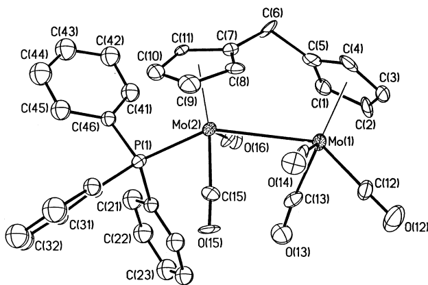
Fig. 1. Molecular structure of (\mu-\eta^5, \eta^5\text{-C}_5\text{H}_4\text{-CH}_2\text{-C}_5\text{H}_4)\text{Mo}_2(\text{CO})_5(\text{PPh}_3) .
