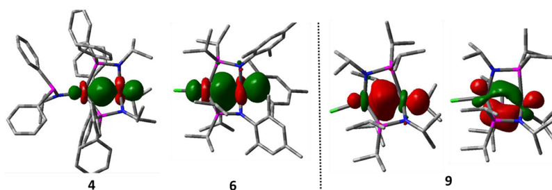
Figure 12. Pictorial representations of the Fe–Fe NBOs of 4 , 6 , and 9 . Composition of Fe–Fe NBO of 4 : 32.3% Fe P (75.8% d, 16.6% p, 7.6% s); 67.7% Fe N (91.2% d, 7.9% s). Composition of Fe–Fe NBO of 6 : 45.3% Fe P (69.6% d, 16.6% p, 13.8% s); 54.7% Fe N (93.0% d, 5.9% s). Composition of Fe–Fe NBOs of 9 : \sigma - 50.9% Fe P (68.1% d, 30.7% s); 49.1% Fe N (48.2% d, 41.0% p, 10.8% s). \pi - 52.2% Fe P (86.1% d, 9.8% p, 4.1% s); 47.8% Fe N (84.2% d, 14.5% p).
