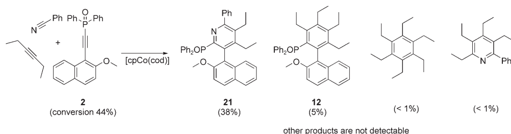
Scheme 4. Three-component cycloaddition.
