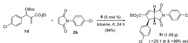
Scheme 3. Gram Scale [3 + 2] Annulation between MBH Carbonate 1d and Maleimide 2b
