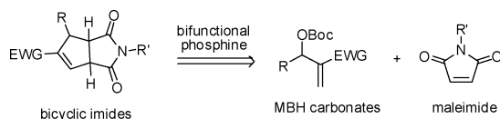
Scheme 1. Construction of Bicyclic Imides via Phosphine Catalyzed [3 + 2] Annulation
