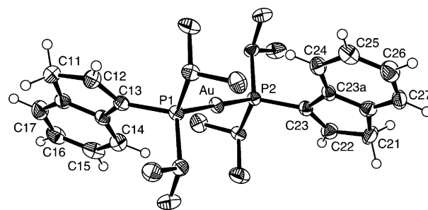
Figure 4. ORTEP diagram for [7]^+\text{OTf}^- shown with 50% displacement ellipsoids and with the atomic numbering scheme depicted; selected hydrogen atoms and the triflate counterion have been omitted for clarity. Selected interatomic distances (Å) and angles (deg) for [7]^+\text{OTf}^- : Au–P1 2.310(1); Au–P2 2.315(1); P1–C13 1.800(4); P2–C23 1.804(4); C11–C12 1.507(7); C12–C13 1.326(7); C21–C22 1.483(7); C22–C23 1.333(7); and P1–Au–P2 179.26(4).
