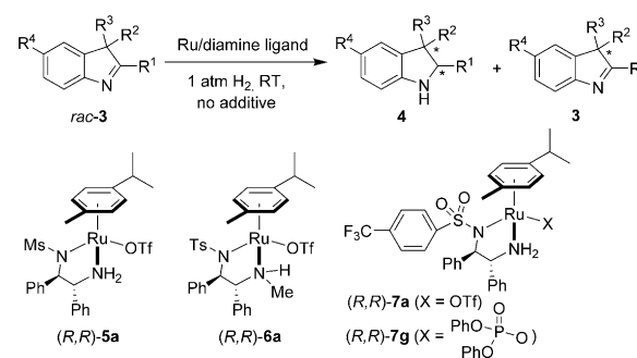
Scheme 1. Enantioselective synthesis of indolines by AH. Boc = tert -butoxycarbonyl, Tf = trifluoromethanesulfonyl, Ts = 4-toluenesulfonyl.
