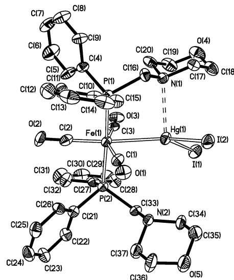
Fig. 2. Perspective view (35% thermal ellipsoids) of [Fe(μ-L) 2 (CO) 3 ]HgI 2 ( 2 ).
