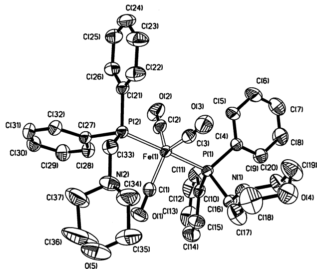
Fig. 1. Perspective view (35% thermal ellipsoids) of trans - [\text{Fe}(\mu\text{-L})_2(\text{CO})_3] ( 1 ). In this and all other figures, the hydrogen atoms have been omitted for clarity.
