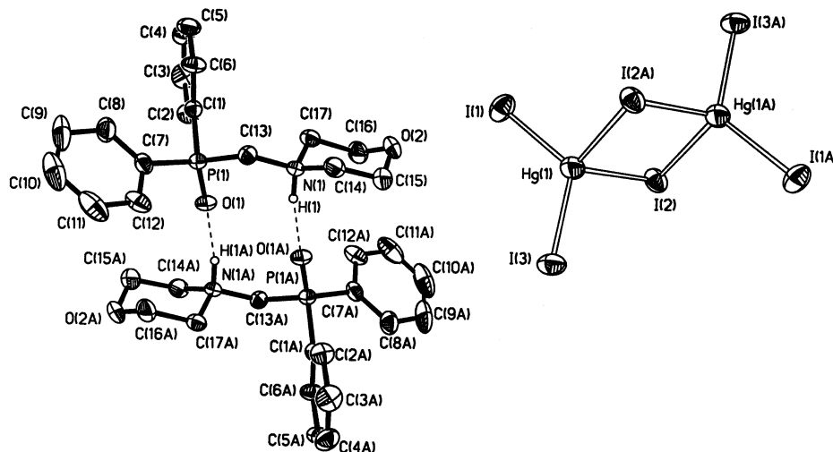
Fig. 5. Perspective view (35% thermal ellipsoids) of the dimeric cationic and anionic species in compound 6 . The N–H···O hydrogen bonds are represented by broken lines.
