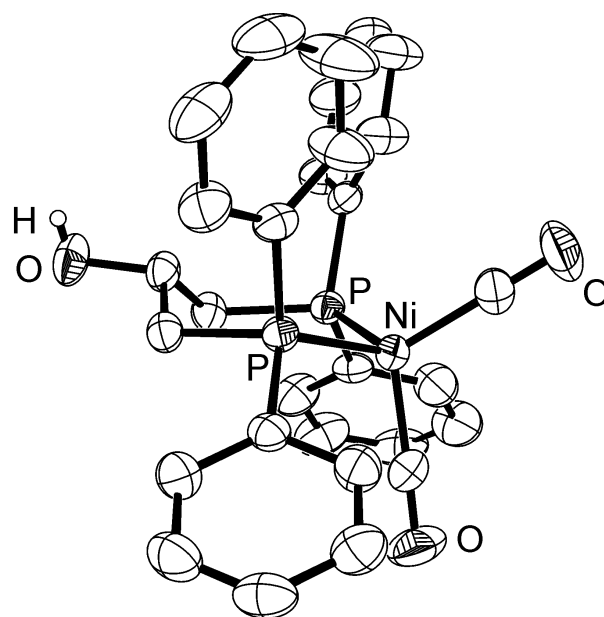
Figure 2. Molecular structure of 13 . Anisotropic replacement parameters are shown at 50% probability level, hydrogen atoms except OH have been omitted for clarity. Details of measurement see ref. [64] Selected angles [°] and bond lengths [Å]: P–Ni–P 101.35(2); C–Ni–C 114.46(10); P–Ni–C 107.20(7)/105.82(7)/114.24(7)/114.46(10); Ni–C 1.768(2)/1.774(2); Ni–P 2.1888(6)/2.1953(6).
