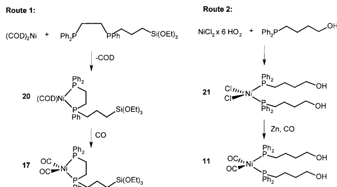
Scheme 3. Two possible routes for the synthesis of carbonylnickel phosphine complexes.
