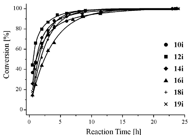
Figure 8. Comparison of the catalytic activities of 10i , 12i , 14i , 16i , 18i , and 19i at 155 °C. For 17i see ref. [12]
