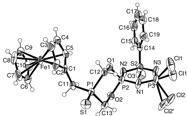
Fig. 1. Molecular structure of \text{FcCH}_2\text{P}(\text{S})(\text{CH}_2\text{O})_2\text{PN}(\text{NPCl}_2)[\text{NS}(\text{O})\text{Ph}] ( 8 ).
