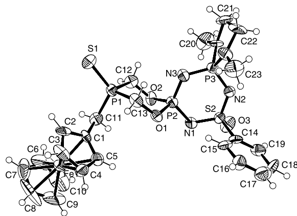
Fig. 2. Molecular structure of \text{FcCH}_2\text{P}(\text{S})(\text{CH}_2\text{O})_2\text{PN}_2\text{P}[\text{N}(\text{Me})\text{CH}_2]_2[\text{NS}(\text{O})\text{Ph}] ( 10 ).
