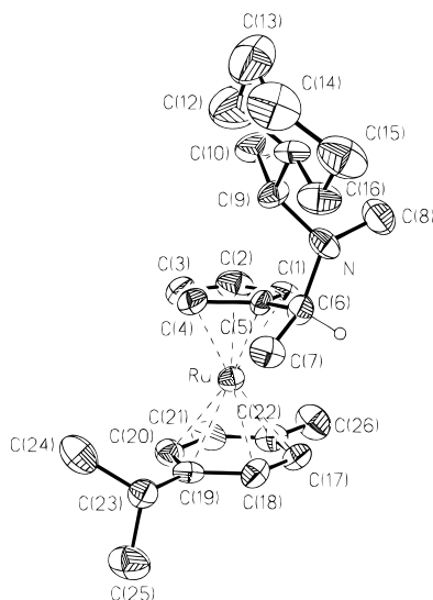
Figure 1. ORTEP view of the cation ( S,R )- 5 (30% probability ellipsoids). The Ru atom is located at 1.831 Å from the Cp ring and 1.703 Å from the p -cymene ring. The planes of the two rings subtend an angle of 3.8°.
