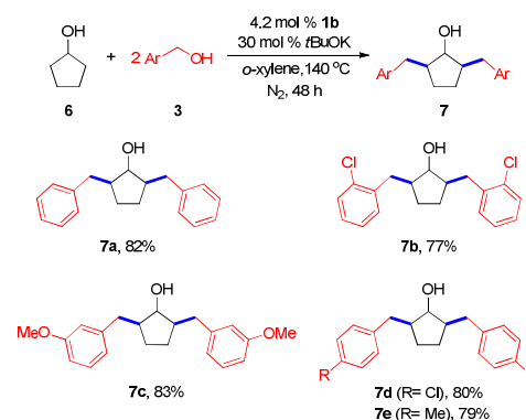
Scheme 4. Reactions of Cyclopentanol with Benzylic Alcohols
