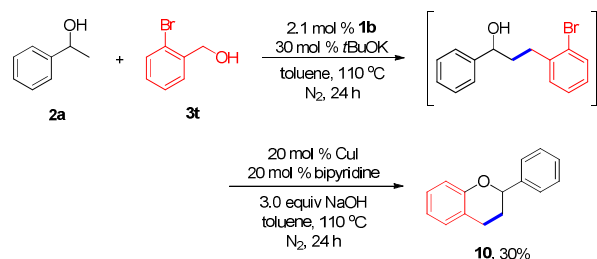
Scheme 5. One-Pot Synthesis of Flavan Derivative 10
