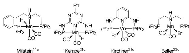
Scheme 1. Selected Known Manganese Complex Catalysts
