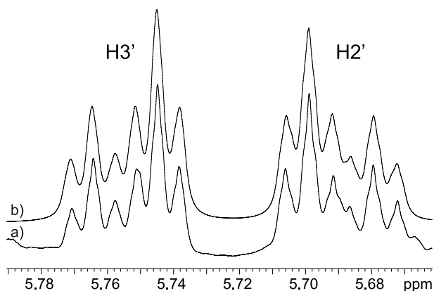
Figure 3. Part of ^1\text{H} NMR spectra of 14 showing \text{H}3' and \text{H}2' multiplets. (a) Experimental spectrum acquired in \text{DMSO}-d_6 at 298 K; (b) simulated spectrum (A2BCD2 spin system).
