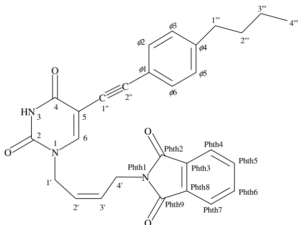
Figure 2. Atom numbering given in Table 1 is exemplified on compound 6 . Note that chemical shifts are equal for \phi 2 and \phi 6 , \phi 3 and \phi 5 , Phth2 and Phth9, Phth3 and Phth8, Phth4 and Phth7, Phth5 and Phth6 due to symmetry.
