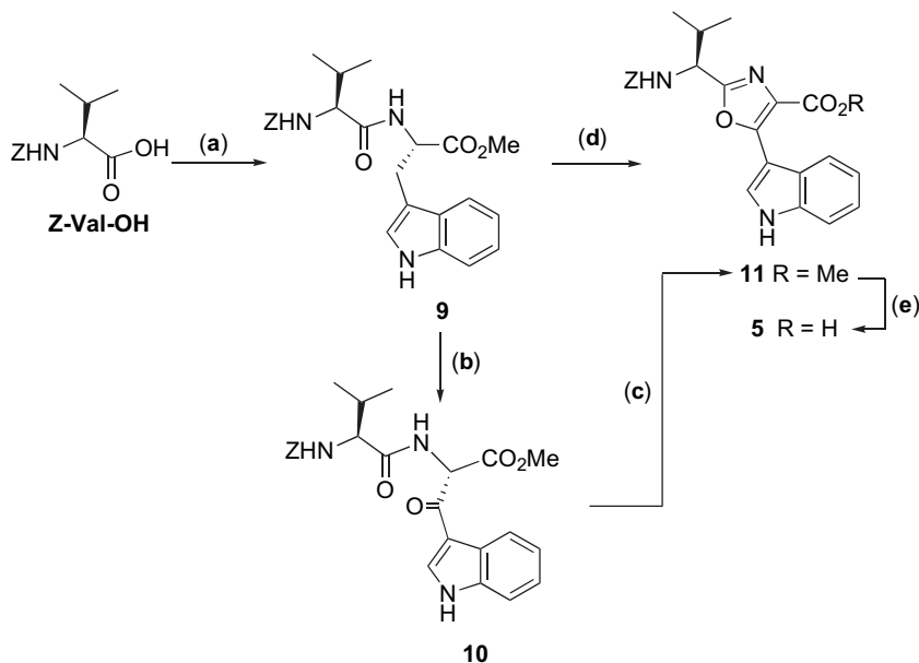
Scheme 3. Reagents and conditions: (a) H-Trp-OMe hydrochloride, HBTU, HOBt, i -Pr 2 NEt, CH 2 Cl 2 , rt, 12 h, 85%; (b) DDQ, THF/H 2 O (9:1), rt, 3 h, 50%; (c) PPh 3 , I 2 , Et 3 N, CH 2 Cl 2 , rt, 3 h, 69%; (d) DDQ, THF, reflux, 3 h, 64%; (e) LiOH, MeOH/H 2 O, rt, 16 h, 82%.
