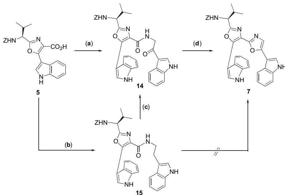
Scheme 5. Reagents and conditions: (a) aminoketone 6 , HBTU, HOBT, i -Pr 2 NEt, CH 2 Cl 2 , rt, 12 h, 42%; (b) tryptamine, HBTU, HOBT, i -Pr 2 NEt, CH 2 Cl 2 , rt, 12 h, 78%; (c) DDQ, THF/H 2 O (9:1), rt, 3 h, 83%; (d) PPh 3 , C 2 Cl 6 , Et 3 N, THF, rt, 30 h, 48%.
