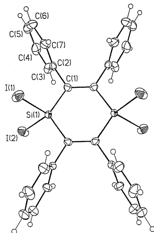
Fig. 5. Computer drawing of the molecular structure
