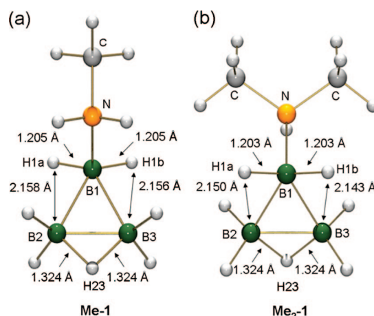
Figure 6. DFT-optimized structures of \text{MeNH}_2\text{B}_3\text{H}_7 (a, Me-1 ) and \text{Me}_2\text{NHB}_3\text{H}_7 (b, Me 2 -1 ).
