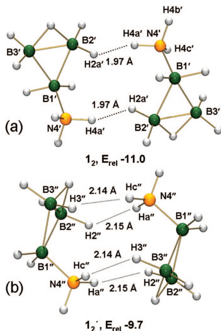
Figure 4. B3LYP-optimized dimeric structures of 1 : (a) 1 2 and (b) 1 2 ' . The MP2/6-311+G(2d,p)-calculated energies are in kcal/mol and are based on the B3LYP/6-31G(d)-optimized structures relative to two separated \text{NH}_3\text{B}_3\text{H}_7 molecules. Selected intermolecular distances and angles. 1 2 : \text{H}2\text{a}'\text{--H}4\text{a}' , 1.97 and 1.97 Å; \text{B}2\text{--H}2\text{a}'\text{--H}4\text{a}' , 100.5° and 100.5°; \text{H}2\text{a}'\text{--H}4\text{a}'\text{--N}4' , 142.2° and 142.2°. 1 2 ' : \text{H}2''\text{--H}a'' , 2.15 and 2.15 Å; \text{H}3''\text{--H}c'' , 2.14 and 2.14 Å; \text{B}2''\text{--H}2''\text{--H}a'' , 118.9° and 119.4°; \text{H}2''\text{--H}a''\text{--N}4'' , 146.0° and 146.4°; \text{B}3''\text{--H}3''\text{--H}c'' , 118.9° and 118.9°; \text{H}3''\text{--H}c''\text{--N}4'' , 146.7° and 147.0°.
