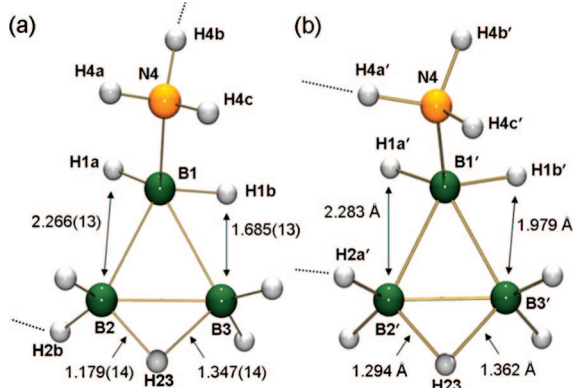
Figure 5. Comparison of (a) the solid-state structure of 1 with (b) the DFT-optimized 1 2 structure. Dashed lines indicate the positions of the dihydrogen bonding interactions.
