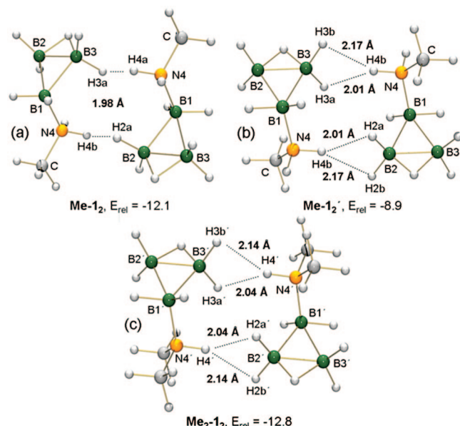
Figure 7. DFT-optimized dimeric structures of (a) (\text{MeNH}_2\text{B}_3\text{H}_7)_2 , \text{Me-1}_2 , (b) (\text{MeNH}_2\text{B}_3\text{H}_7)_2 , \text{Me-1}_2' , and (c) (\text{Me}_2\text{NHB}_3\text{H}_7)_2 , \text{Me}_2\text{-1}_2 . The MP2/6-311+G(2d,p)-calculated energies are in kcal/mol and are based on the B3LYP/6-31G(d)-optimized structures relative to 2 equiv of \text{MeNH}_2\text{B}_3\text{H}_7 and \text{Me}_2\text{NHB}_3\text{H}_7 , respectively.
