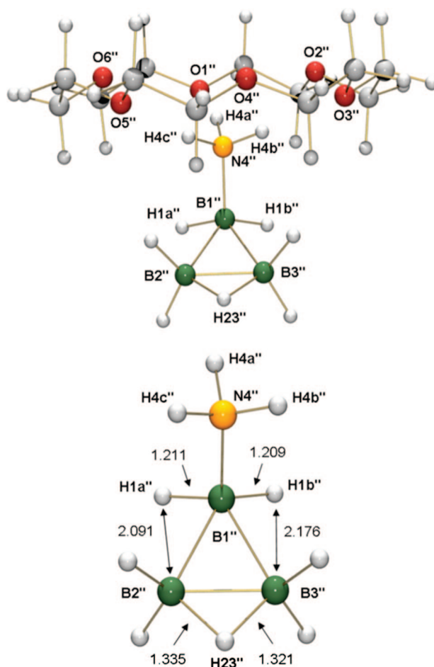
Figure 10. (top) DFT-optimized structure of 1 ·18-crown-6 (molecule a); (bottom) selected calculated distances in the ammonia-triborane fragment of 1 ·18-crown-6 (molecule a).
