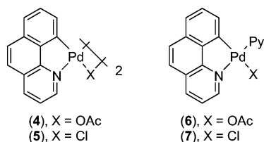
Figure 2. Benzo[ h ]quinoline complexes examined in amination reactions.
