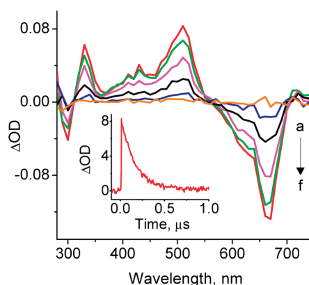
Figure 2. Transient absorption spectra of 5b following 355 nm laser pulse excitation; time-resolved absorption spectra recorded at (a) 0.1, (b) 0.4, (c) 1, (d) 2, (e) 4, and (f) 10 \mu\text{s} . Inset shows the decay of the transient at 510 nm.
