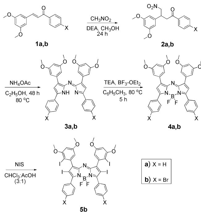
Scheme 1. Synthesis of Aza-BODIPY Derivatives
