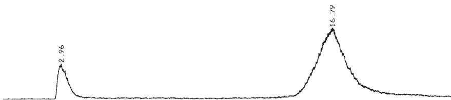
Figure 1. Radiochromatogram of a [ 123 I]-4-iodo- N -(4-(4-(2-methoxyphenyl)-piperazin-1-yl)butyl)-benzamide ( 123 I-1) synthesis
