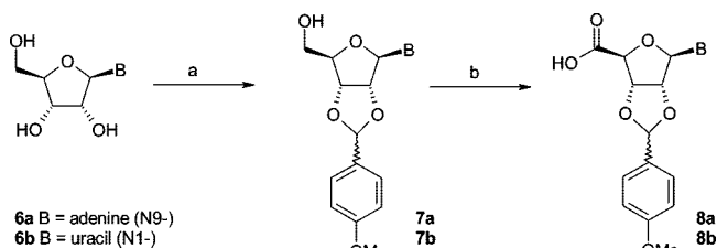
Scheme 1. Synthesis of 2',3'-Protected Nucleoside-5'-Carboxylic Acids a
