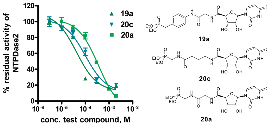
Figure 3. Concentration–inhibition curves of selected inhibitors at NTPDase2. The enzyme assays were performed in a final volume of 100 \mu L using a substrate (ATP) concentration of 400 \mu M ( K_m = 70 \mu M). Product formation was determined by capillary electrophoresis as described in the Experimental Section. Data points represent the mean \pm SEM from two separate experiments each performed in triplicate. Determined IC_{50} values were 42 \mu M ( 19a ), 101 \mu M ( 20c ), and 374 \mu M ( 20a ). Calculated K_i values were 8.2 \mu M ( 19a ), 29.2 \mu M ( 20c ), and 71.7 \mu M ( 20a ).
