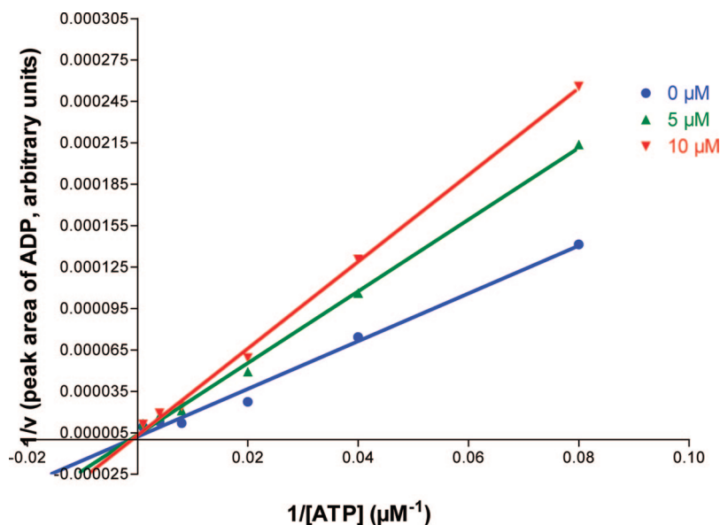
Figure 4. Lineweaver–Burk plot for NTPDase2 kinetics in the absence and in the presence of two different concentrations of the inhibitor 19a (5 and 10 \mu M).
