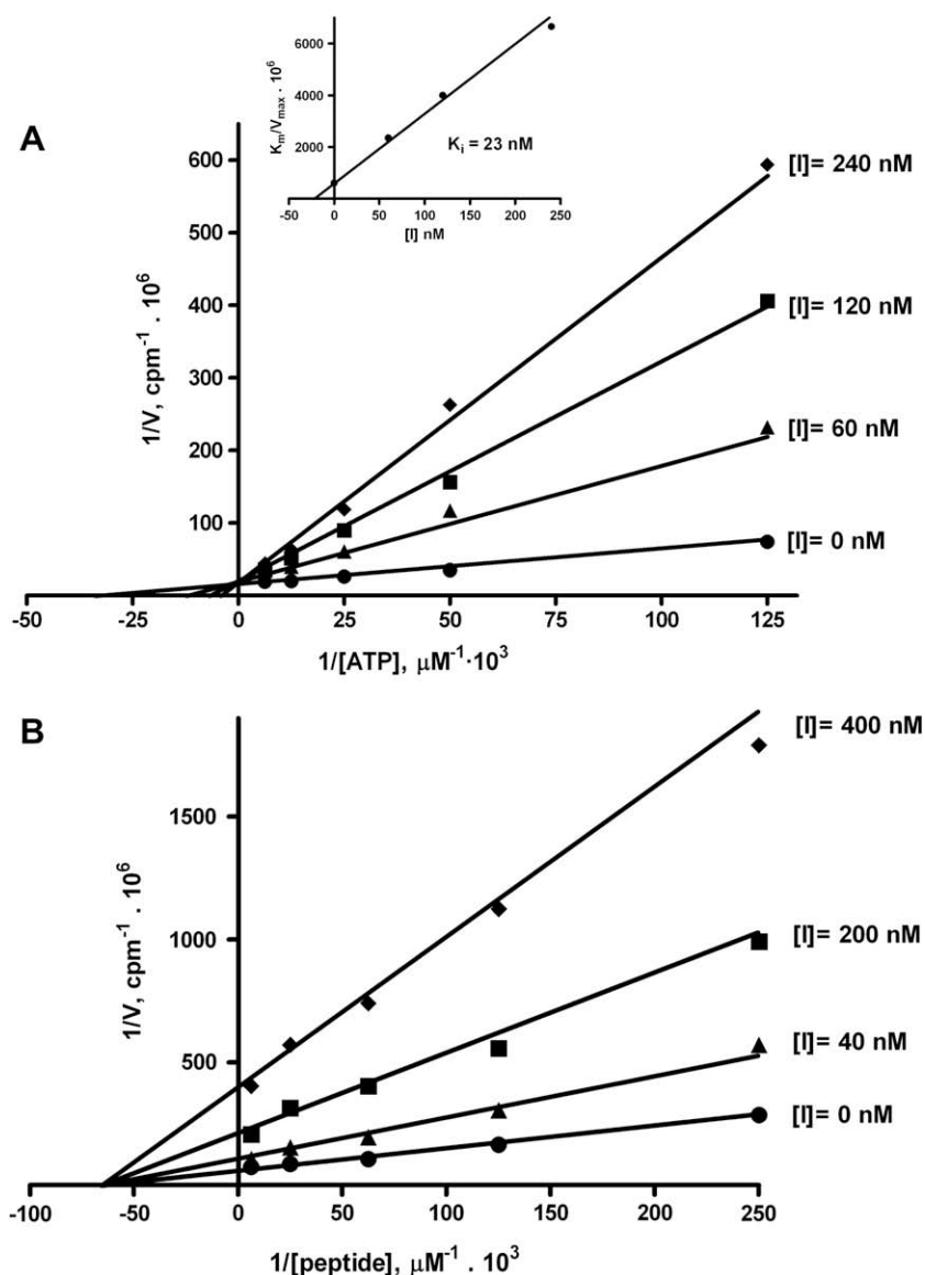
Figure 1. Double-reciprocal plot analysis of CK2 inhibition by compound 1a (TIBI). CK2 activity was determined as described in Section 3 either in the absence or in the presence of the indicated fixed concentrations of inhibitor. In A the concentration of the peptide substrate was constant (100 \mu M) at increasing concentrations of ATP while in B the ATP concentration was constant (80 \mu M) at increasing concentrations of peptide substrate. The data represent the mean of triplicate experiments with SEM never exceeding 15%. The K_i of the inhibitor competitive with respect to ATP was then calculated by linear regression analysis of K_m/V_{max} versus inhibitor concentration plot shown in the inset of panel A.
