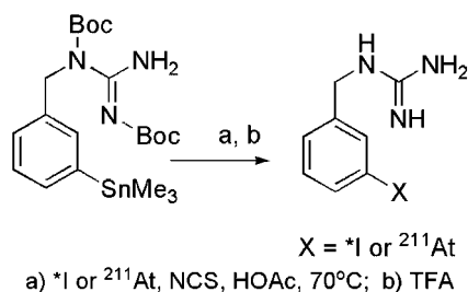
Figure 2 Radiohalogenation of the tin precursor to [ ^*\text{I} ]MIBG and [ ^{211}\text{At} ]MABG.
