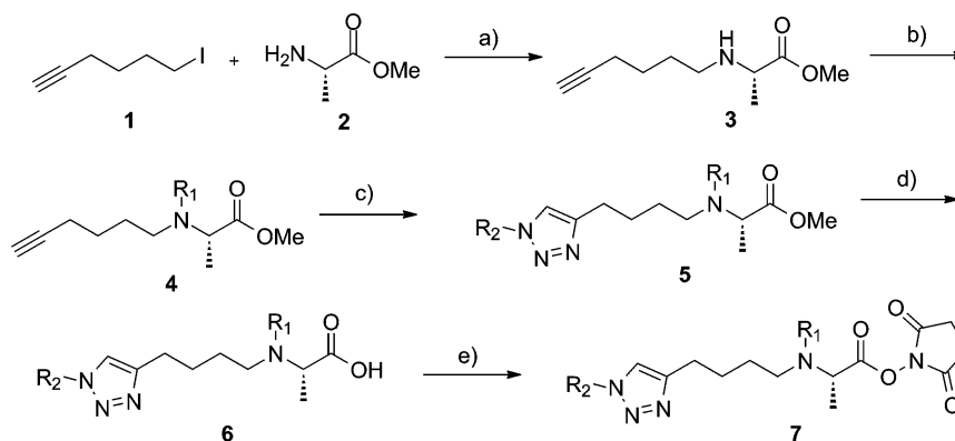
Figure 1. Synthesis of CIT reagents. (a) THF, K 2 CO 3 , TEAL, reflux 18 h, 56%. (b) THF, K 2 CO 3 , TEABr, reflux 18 h, R 1 = Allyl- d 0 -bromide (4a), 56%, R 1 = Allyl- d 5 -bromide (4b), 67%. (c) 0.4 equiv Na ascorbate, 0.1 equiv CuSO 4 , 0.01 equiv TBTA, DMSO/H 2 O, RT 4 h, R 2 = Allyl- d 5 -azide (5a), 72% (heavy tag), R 2 = Allyl- d 0 -azide (5b), 69% (light tag). (d) 2 M KOH, THF, RT overnight, quantitative (heavy tag, 6a), 97% (light tag, 6b). (e) TFA-NHS, DMF, RT overnight, 24% (heavy tag, 7a), 23% (light tag, 7b). THF = tetrahydrofuran, TEAL = tetraethylammonium iodide, TEABr = tetraethylammonium bromide, TBTA = tris[(1-benzyl-1 H -1,2,3-triazol-4-yl)methyl]amine, DMSO = dimethyl sulfoxide, TFA-NHS = trifluoroacetic N -hydroxysuccinimide ester, DMF = N,N -dimethyl formamide.
