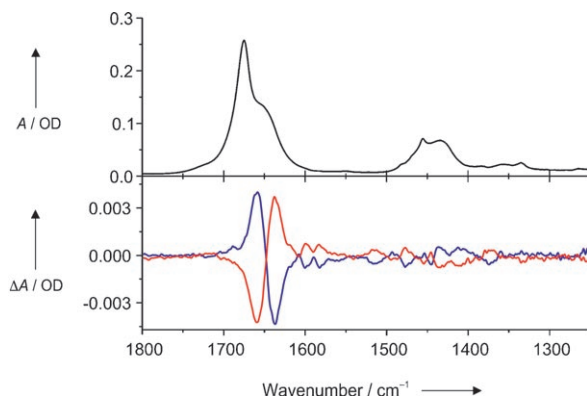
Figure 8. Top: FTIR-absorption spectrum of the AMPP-peptide at 25^{\circ}\text{C} ; bottom: Absorption difference spectra induced by irradiation at 355\text{ nm} ( trans \rightarrow cis , red curve) and at \lambda > 400\text{ nm} ( cis \rightarrow trans , blue curve). The strong absorption changes around 1650\text{ cm}^{-1} are due to the different \beta -hairpin content of the cis -azo and trans -azo isomer.
