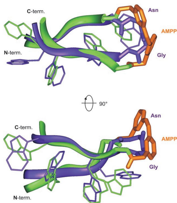
Figure 4. Backbone superimposition of the energy lowest NMR structure of the AMPP-peptide as cis -azo isomer (green ribbons) on the original tryptophan zipper (violet ribbons, PDB code: 1LE1). The AMPP chromophore is colored in orange and side chains of only the tryptophan residues are depicted for both peptides. The two views are rotated by 90° around a horizontal axis.
