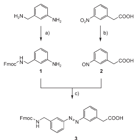
Scheme 1. Synthesis of the N-Fmoc-protected photoswitch [3-(3-aminomethyl)phenylazo]phenylacetic acid (AMPP). a) Fmoc-OSu, \text{Et}_3\text{N} , RT; b) \text{NH}_4\text{Cl} , Zn powder, RT; then \text{FeCl}_3 , 0 °C; c) AcOH.
