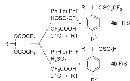
Scheme 1. Synthesis of FITS ( 4a ) and FIS ( 4b )-type reagents from perfluoroalkyliodides ( \text{R}^3 = \text{H}, \text{F}; \text{R}_f (n\text{-C}_m\text{F}_{2m+1}): m = 10, 8, 7, 6, 3, 2; \text{or } i\text{-C}_3\text{F}_7 ).
