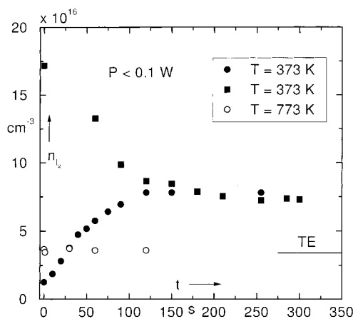
Figure 9. Temporal development of the CEEC ( I_2 component) in a Tesla spark discharge at different gas temperatures and initial concentrations: (Full squares) T = 373 K, n_{I_{20}} = 1.6 \times 10^{17} \text{ cm}^{-3} , n_{H_{20}} = 2.1 \times 10^{17} \text{ cm}^{-3} , n_{HI0} = - \text{cm}^{-3} , n_{He} = 2 \times 10^{19} \text{ cm}^{-3} ; (full circles) T = 373 K, n_{I_{20}} = 2.9 \times 10^{16} \text{ cm}^{-3} , n_{H_{20}} = 6.3 \times 10^{16} \text{ cm}^{-3} , n_{HI0} = 2.6 \times 10^{17} \text{ cm}^{-3} , n_{He} = 2 \times 10^{19} \text{ cm}^{-3} ; (open circles) T = 773 K, n_{I_{20}} = 2.9 \times 10^{16} \text{ cm}^{-3} , n_{H_{20}} = 6.3 \times 10^{16} \text{ cm}^{-3} , n_{HI0} = 2.6 \times 10^{17} \text{ cm}^{-3} , n_{He} = 2 \times 10^{19} \text{ cm}^{-3} ; (line) composition according to the thermodynamic equilibrium (TE) for T = 773 K.
