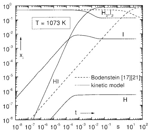
Figure 11. Temporal development of the product composition of the thermodynamic equilibrium calculated by the kinetic model (see Table 2) as well as by the gross reaction 1. 17
