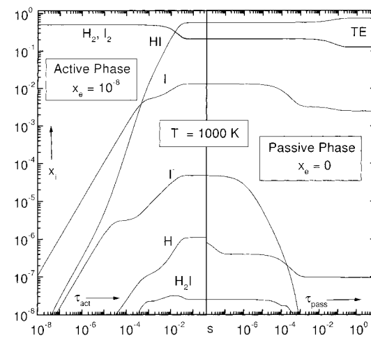
Figure 13. Temporal development of the gas composition at T = 1000 K for a stoichiometric input mixture ( x I20 = x H20 = 0.5).
