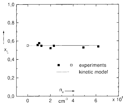
Figure 8. Dependence of the relative I 2 concentration on the average concentration of plasma electrons: reactor diameter: 9 mm; length: 120 mm; tube temperature: 360 K; (open square) Tesla spark discharge ( P < 0.1 W); (filled squares) rf discharge (450–610 kHz); input mixture x_{I_{20}} = 0.61 , x_{H_{20}} = 0.39 ; total particle number density: n = 4.1 \times 10^{16} \text{ cm}^{-3} .
