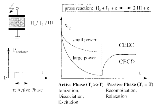
Figure 1. Occurrence of chemical quasi-equilibria in a closed system (illustration for the gross reaction \text{H}_2 + \text{I}_2 + e \rightleftharpoons 2\text{HI} + e ).
