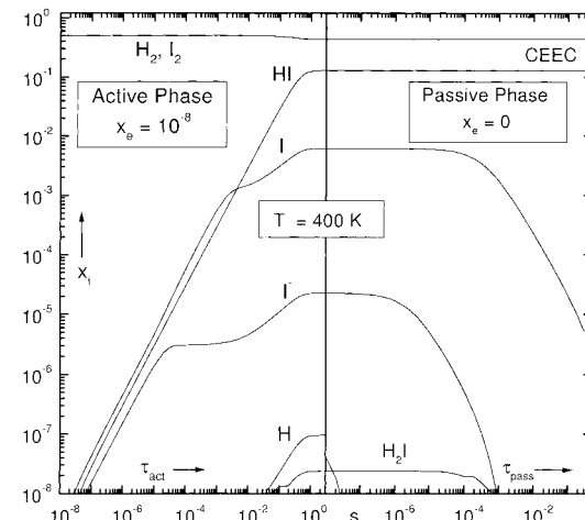
Figure 14. Temporal development of the gas composition at T = 400 K for a stoichiometric input mixture ( x I20 = x H20 = 0.5).
