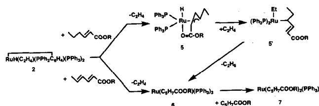
Scheme 1. A reaction mechanism of 2 with alkyl 2-hexenoate.
