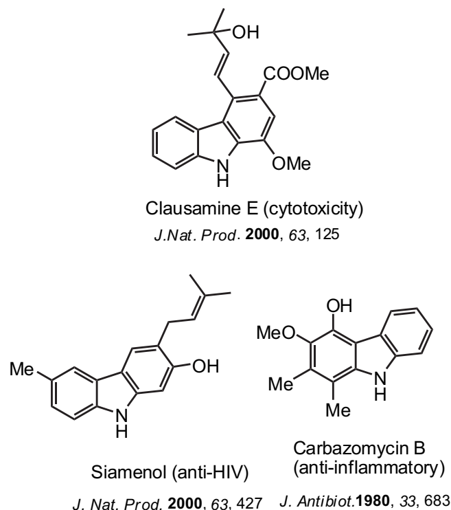
Fig. 1. Natural carbazoles.
