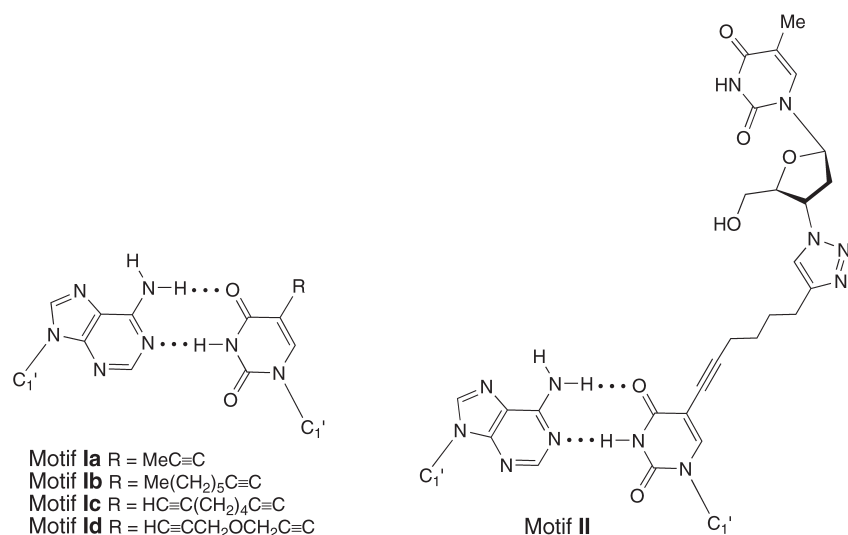
Fig. 6. Base-pair motifs formed by 1a–d and 6
