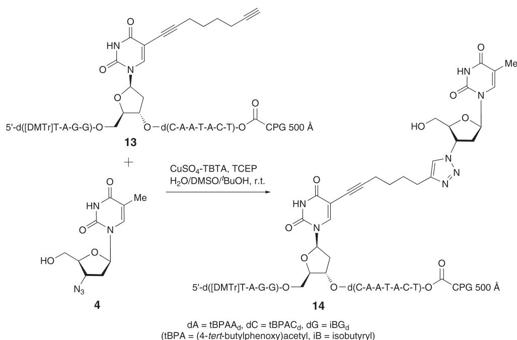
Scheme 5. Cycloaddition Performed with the Oligonucleotide 13
