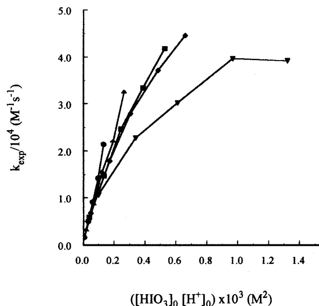
Figure 3. Saturation of k_{\text{exp}}/10^4 \text{ (M}^{-1} \text{ s}^{-1}\text{)} with increasing ([\text{HIO}_3]_0 [\text{HClO}_4]_0) \times 10^3 \text{ (M}^2\text{)} over the range 0.0968 \text{ M} \leq [\text{HClO}_4]_0 \leq 0.489 \text{ M} in five series of experiments at constant [\text{KIO}_3]_0 of (●) 0.000\,448 \text{ M} , (▲) 0.000\,896 \text{ M} , (■) 0.001\,79 \text{ M} , (◆) 0.002\,24 \text{ M} , and (▼) 0.004\,48 \text{ M} .
