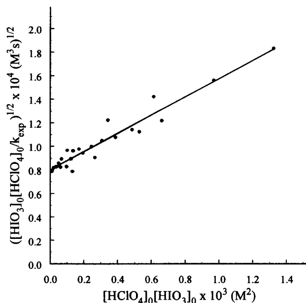
Figure 4. Plot of ([\text{HIO}_3]_0 [\text{HClO}_4]_0 / k_{\text{exp}})^{1/2} \times 10^4 \text{ (M}^3 \text{ s)}^{1/2} vs ([\text{HIO}_3]_0 [\text{HClO}_4]_0) \times 10^3 \text{ (M}^2\text{)} according to eq 7. Slope = k^*/k^{1/2} = (7.8 \pm 0.4) \times 10^{-2} \text{ (s/M)}^{1/2} = (K_9 K_{10}/k_{11})^{1/2} and intercept = 1/k^{1/2} = (8.0 \pm 0.2) \times 10^{-5} \text{ (M}^3 \text{ s)}^{1/2} = (1/K_9 K_{10} k_{11})^{1/2} .
