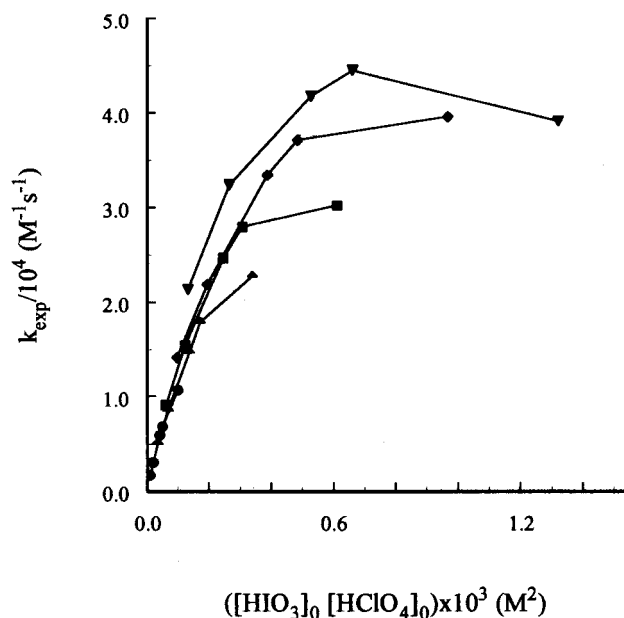
Figure 2. Saturation of k_{\text{exp}}/10^4 \text{ (M}^{-1} \text{ s}^{-1}\text{)} with increasing ([\text{HIO}_3]_0 [\text{HClO}_4]_0) \times 10^3 \text{ (M}^2\text{)} over the range 0.000\,448 \text{ M} \leq [\text{KIO}_3]_0 \leq 0.004\,48 \text{ M} in five series of experiments at constant [\text{HClO}_4]_0 of (●) 0.0968 \text{ M} , (▲) 0.199 \text{ M} , (■) 0.289 \text{ M} , (◆) 0.393 \text{ M} , and (▼) 0.489 \text{ M} .
