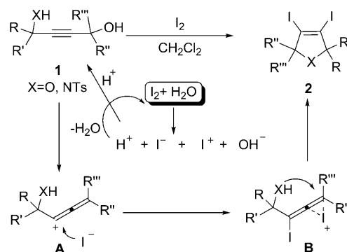
Scheme 4. Proposed mechanism.
