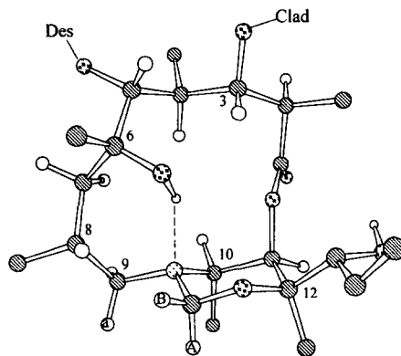
Figure 2. Modeled, representative conformation of structure 24 derived from the NOE data. The aglycone and hydroxyl protons are shown as unshaded circles.
