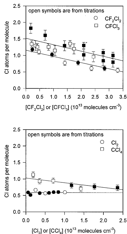
Figure 3. Dissociation efficiency for \text{Cl}_2 , \text{CF}_2\text{Cl}_2 , \text{CFCl}_3 , and \text{CCl}_4 vs precursor concentration. The number of Cl atoms produced per molecule of \text{Cl}_2 is 0.6 for the [\text{Cl}_2] range studied. The apparent dissociation efficiency for the chlorofluoromethanes decreases linearly, with the same apparent slope for increasing precursor concentration. The highest number of Cl atoms per precursor molecule is 1.5, 1.1, and 1.0 for \text{CF}_2\text{Cl}_2 , \text{CFCl}_3 , and \text{CCl}_4 , respectively.
