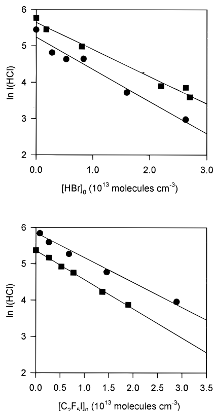
Figure 5. Pseudo-first-order plot of Cl atom concentration vs \text{C}_2\text{F}_5\text{I} concentration. The reaction pressure was 2 Torr, [\text{H}_2\text{S}] = 1 \times 10^{13} \text{ cm}^{-3} , and \Delta t = 11 \text{ ms} . (a) The slope ( \text{cm}^3 \text{ molecule}^{-1} ) and [\text{Cl}]_0 (atoms \text{cm}^{-3} ) for the HBr experiments are as follows: (●) [\text{Cl}]_0 = 6.2 \times 10^{12} , slope = 8.9 \times 10^{-14} ; (■) [\text{Cl}]_0 = 1.2 \times 10^{13} , slope = 7.5 \times 10^{-14} . (b) For \text{Cl} + \text{C}_2\text{F}_5\text{I} : (●) [\text{Cl}] = 6.2 \times 10^{12} , slope = 6.9 \times 10^{-14} ; (■) [\text{Cl}]_0 = 1.2 \times 10^{13} , slope = 8.0 \times 10^{-14} .
