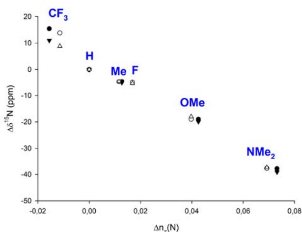
Figure 2. The ^{15}\text{N} NMR chemical shift changes (relative to 1a or 2a , respectively), \Delta\delta^{15}\text{N} , of substituted pyridines (●), of the corresponding 1,2-bis(pyridine-2-ylethynyl)benzene ligands 3a-f (○), and of their [\text{N}-\text{I}-\text{N}]^+ complexes, 1a-d,f (▼) and 2a-f (Δ), respectively, strongly correlate to the corresponding changes in the \pi(\text{N}) orbital population. This indicates that the variation in \delta^{15}\text{N} is dominantly governed by the paramagnetic ring currents in the pyridine moieties.
