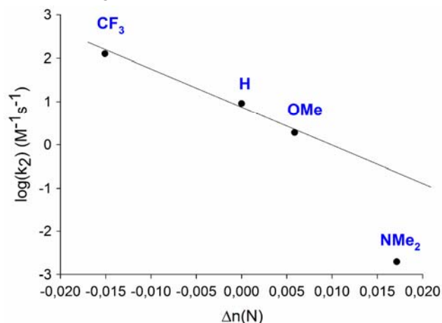
Figure 6. The second-order rate constants ( M^{-1} \times s^{-1} ) of 1a,c,d,f in iodocyclization reactions with 4-penten-1-ol in the presence of 4-R-pyridine ( R = H, OMe, NMe_2 or CF_3 ), normalized to 1 mM, obtained in dry dichloroethane, are shown as a function of the change of natural atomic population, \Delta n(N) . A linear correlation is seen for all but the most electron rich complex 1d .
