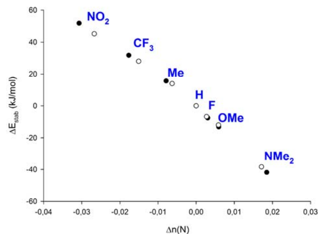
Figure 4. The correlation of the stabilization energy ( \Delta E_{\text{stab}} ) and the change of the natural atom population at the N atoms of the iodine(I) complexes of substituted pyridines ( 1a-g ) (○) and of the corresponding 1,2-bis((pyridine-2-ylethynyl)benzene) ligands ( 2a-g ) (●).
