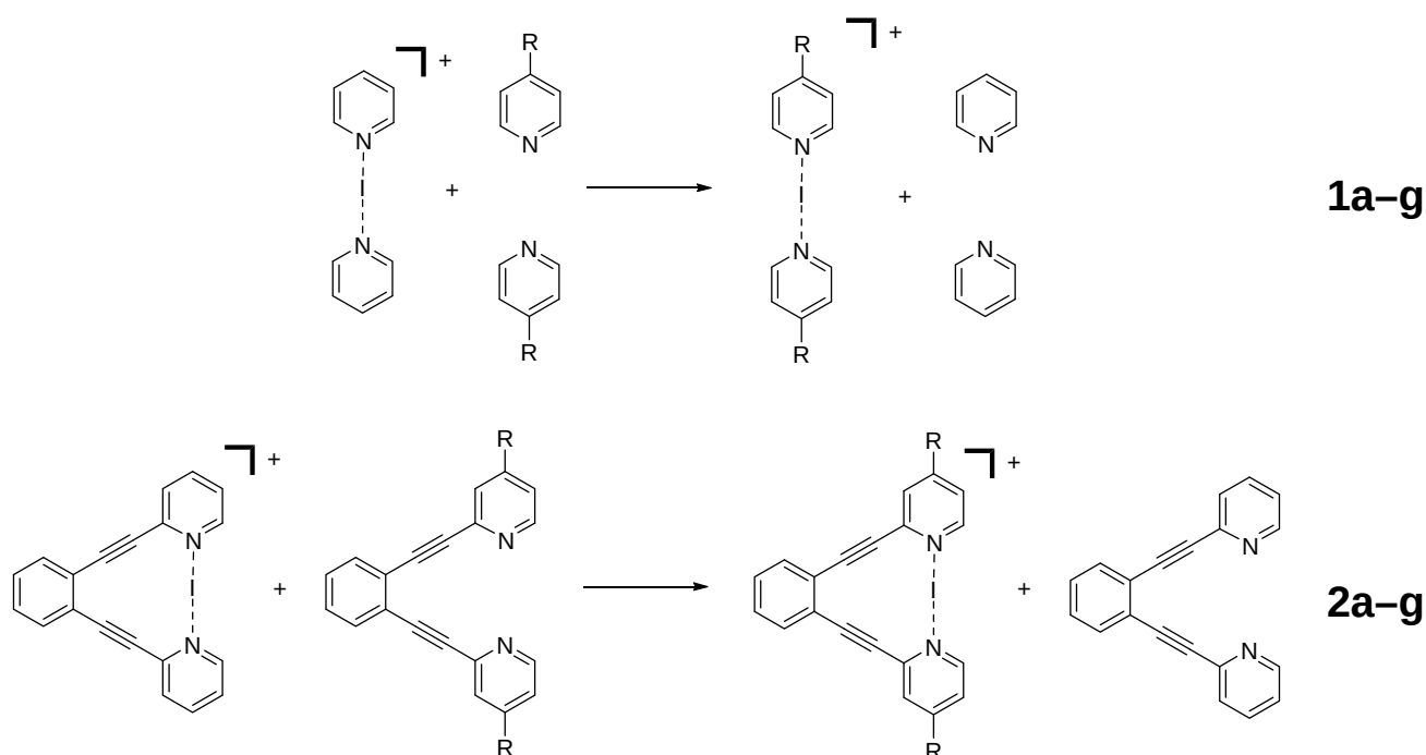
Scheme 4. The formal reactions used to define the stabilization energies of complexes 1a-g and 2a-g .
