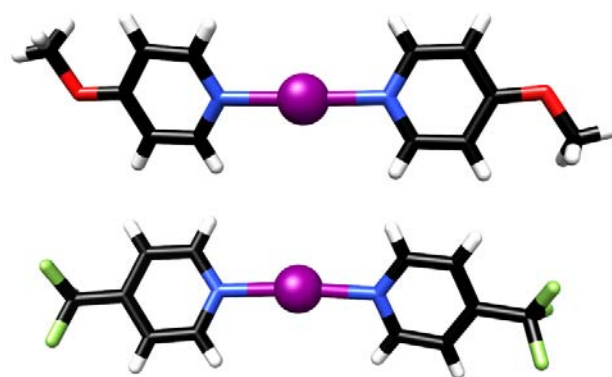
Figure 5. The solid state geometries of complexes 1c (top, CCDC-1452897), and 1f (bottom, CCDC-1452897), obtained by single crystal X-ray crystallography. The \text{BF}_4^- counterion is omitted from the figure for clarity. The crystal of compound 1c was obtained as a solvate and thus each molecular unit contains one molecule dichloroethane. Both complexes possess coplanar pyridine rings and nearly centrosymmetric geometries.
