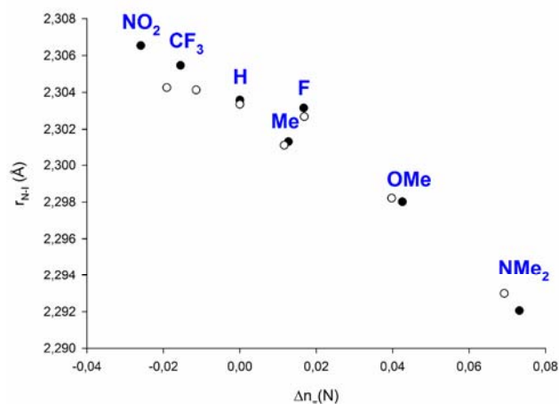
Figure 3. The correlation of the N–I bond distance with the change in the \pi(\text{N}) population of iodine(I) complexes of substituted pyridines ( 1a-g ) (●) and of the corresponding 1,2-bis((pyridine-2-ylethynyl)benzene) ligands ( 2a-g ) (○).
