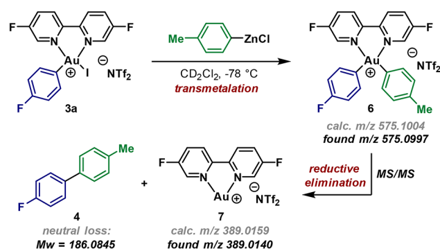
Scheme 5. Transmetalation and Reductive Elimination from 3a
