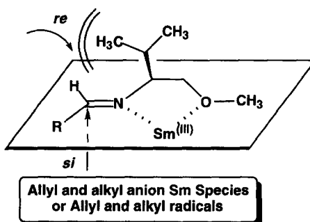
Figure 1. Plausible mechanism of Barbier-type allylation and alkylation with \text{Sm} and iodine (cat.).
