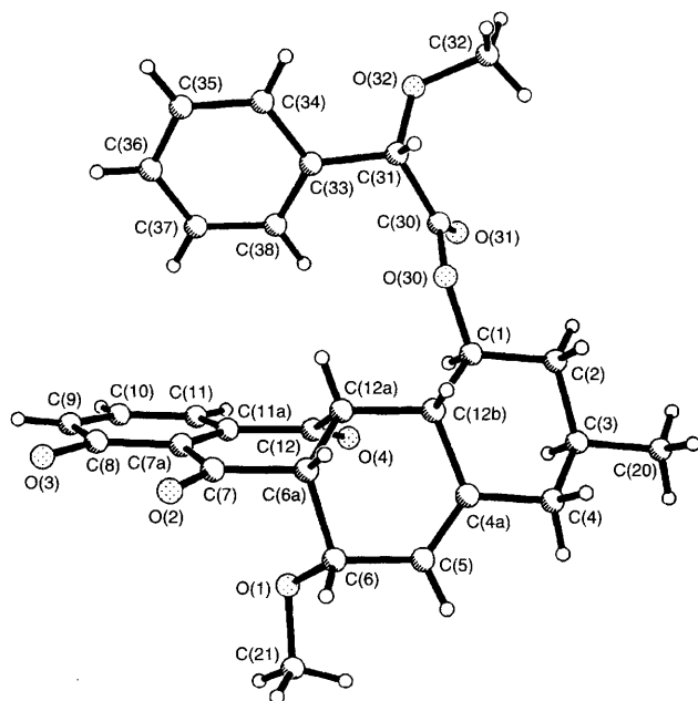
Fig. 2 Molecular structure of 7c
