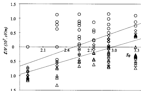
Figure 6. Diagram showing the different reaction products observed behind the reaction fronts propagating toward the positive ( E/V < 0 ) and negative ( E/V > 0 ) electrodes. The symbols \Delta , \diamond , and \circ indicate the assumed net stoichiometries corresponding to the AA-excess, intermediate, and iodate-excess cases respectively, as in Figure 4.
