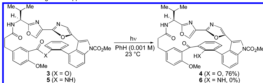
Scheme 2. Methods Used To Form the C10 Quaternary Center in the Three Syntheses of Diazonamide A
