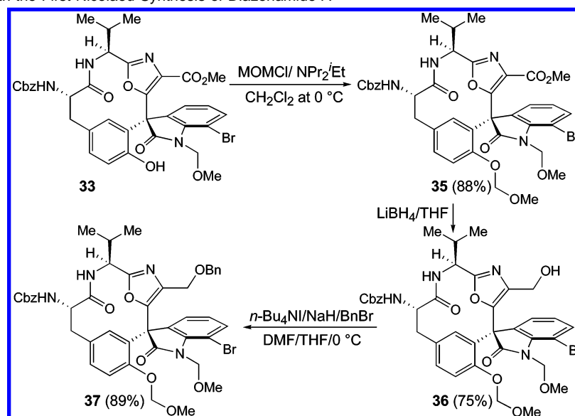
Scheme 6. Correlation with the First Nicolaou Synthesis of Diazonamide A
