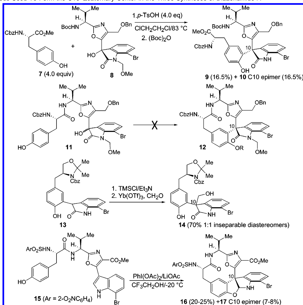
Scheme 2. Methods Used To Form the C10 Quaternary Center in the Three Syntheses of Diazonamide A
