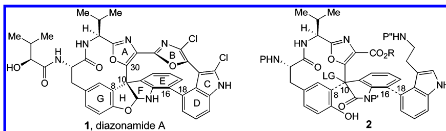
Figure 1. Structure of diazonamide A 1 and crucial disconnections 2 .
