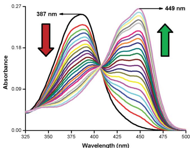
Fig. 1 UV-visible spectral changes of 10 \mu M DMSO solution of receptor 1 upon concomitant additions of Al ^{3+} (0–5 equivalents).
