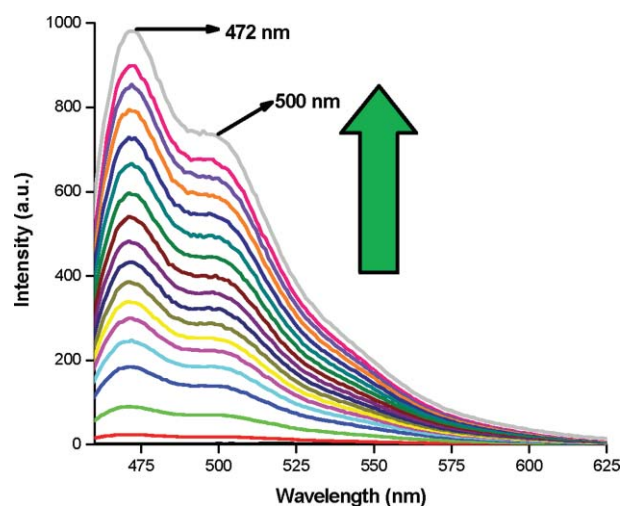
Fig. 2 Fluorescence titration curve of 0.5 \mu M DMSO solution of receptor 1 upon concomitant additions of Al ^{3+} ion (0–3 equivalents).
