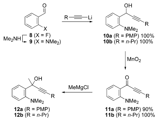
Scheme 3. Preparation of Iodocyclization Precursors
