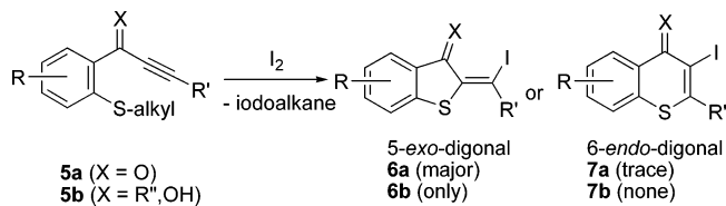
Scheme 2. 5-exo-Digonal and 6-endo-Digonal Cyclization of 5
