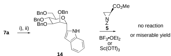
Scheme 5. i) \text{BnBr} , \text{Bu}_4\text{NI} , \text{NaH} , DMF, RT, overnight (87%); ii) 10% NaOH aq, EtOH, reflux, overnight (80%).
