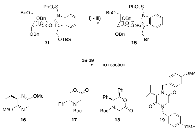
Scheme 6. i) \text{BnBr} , \text{Bu}_4\text{NI} , \text{NaH} , DMF, RT, overnight (85%); ii) \text{TsOH} \cdot \text{H}_2\text{O} , MeOH, RT, 5 h (90%); iii) NBS, \text{PPh}_3 , \text{CH}_2\text{CH}_2 , quant.
