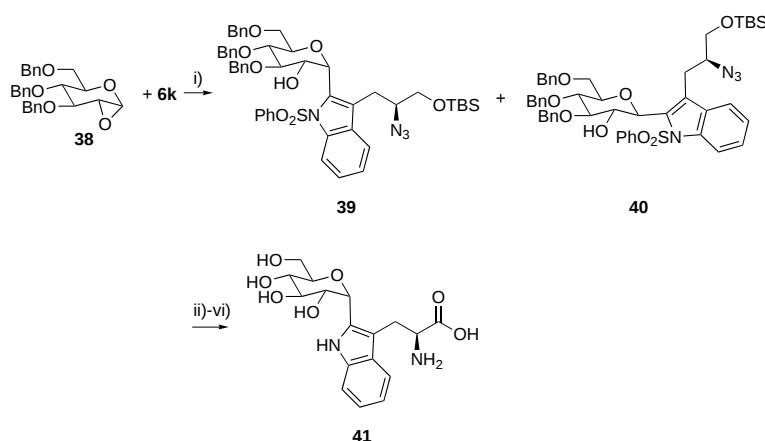
Scheme 13. i) BuLi, \text{BF}_3 \cdot \text{OEt}_2 , THF, 39 (10 %) and 40 (2 %); ii) BnBr, \text{Bu}_4\text{NI} , NaH, THF, 0^\circ\text{C} , RT, overnight (77 %); iii) \text{TsOH} \cdot \text{H}_2\text{O} , MeOH, RT, overnight (99 %); iv) iodosobenzene diacetate, TEMPO, \text{CH}_3\text{CN} , \text{H}_2\text{O} , RT, 3 h (85 %); v) 10 % NaOH, EtOH, reflux, overnight (56 %); v) \text{H}_2 , 20 % \text{Pd}(\text{OH})_2/\text{C} , EtOH, dioxane, \text{H}_2\text{O} (65 %).
